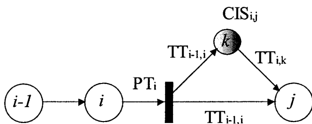
Figure 3. Extended S-graph representation: PT is the task processing time, and TT the transfer times.
