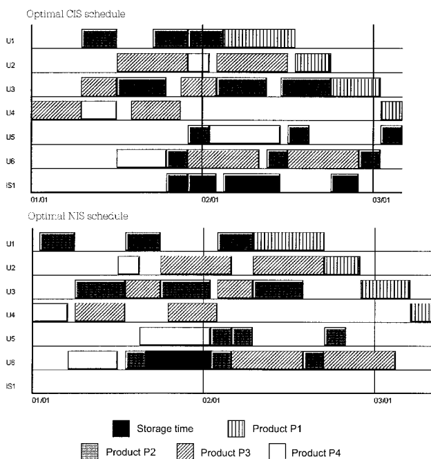
Figure 12. Optimal Gantt charts of multipurpose Example 2 when scheduling one batch of product A, three of B, two of C, and one of D, when a common storage unit is available, and when no storage unit is available.
