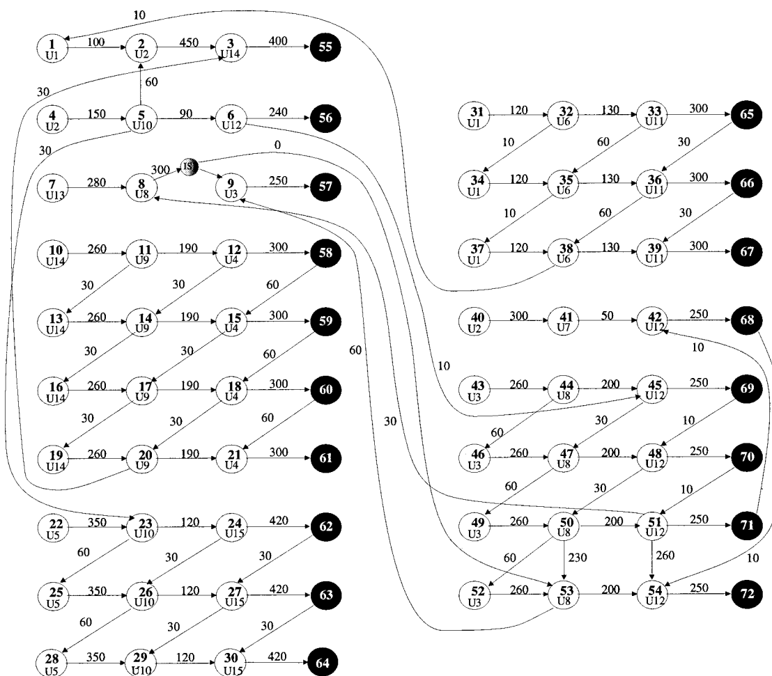
Figure 15. Schedule graph of the optimal CIS solution of Example 4.
