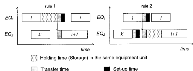
Figure 6. Gantt-chart of the situations found in the non-necessity rules 1 and 2.
