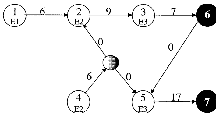
Figure 5. Feasible schedule graph of the case in Figure 4 thanks to the introduction of an intermediate storage; C-type nodes are omitted.
