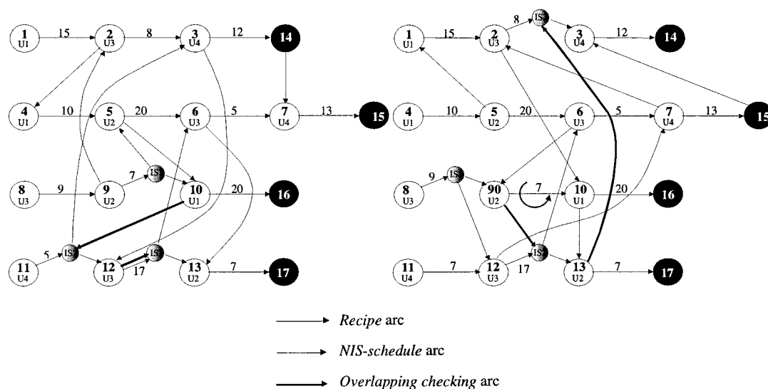
Figure 14. Infeasible schedule graph representation of the solution proposed by Kim et al. (2000) and optimal feasible schedule graph according to the S-graph algorithm.
