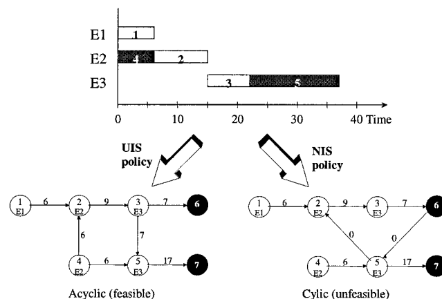
Figure 4. S-graph representation of UIS and NIS policy of a batch process.
