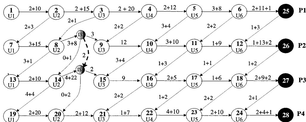
Figure 11. Optimal schedule graph of multiproduct Example 1; the weight of the arcs show the processing times, transfer times, and setup times.
