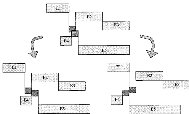
Figure 8. Case where the addition of overlapping-checking arcs does not generate a cycle but modifies makespan.
