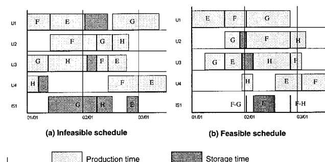
Figure 13. Infeasible optimal Gantt chart proposed by Kim et al. (2000) and optimal feasible Gantt chart according to the S-graph algorithm.
