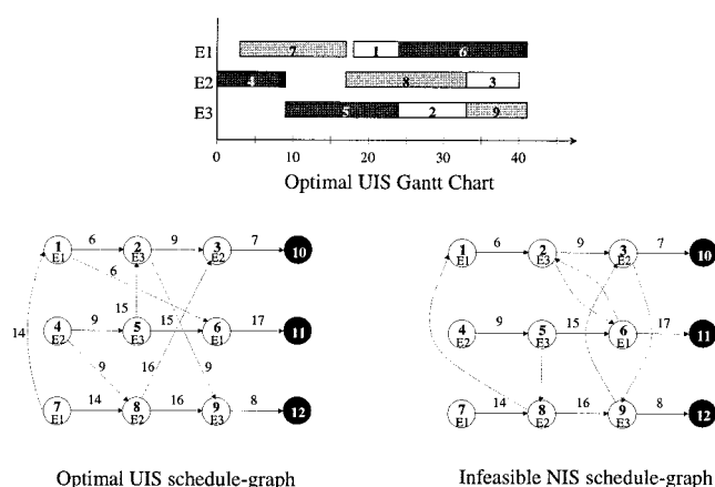
Figure 2. Optimal UIS and its corresponding NIS policies S-graph representation of a batch process.
