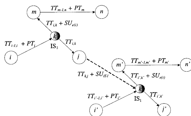
Figure 7. Possibility of intermediate storage unit use. PT is the task processing time, TT the transfer time and SU, the setup time of an equipment unit.
